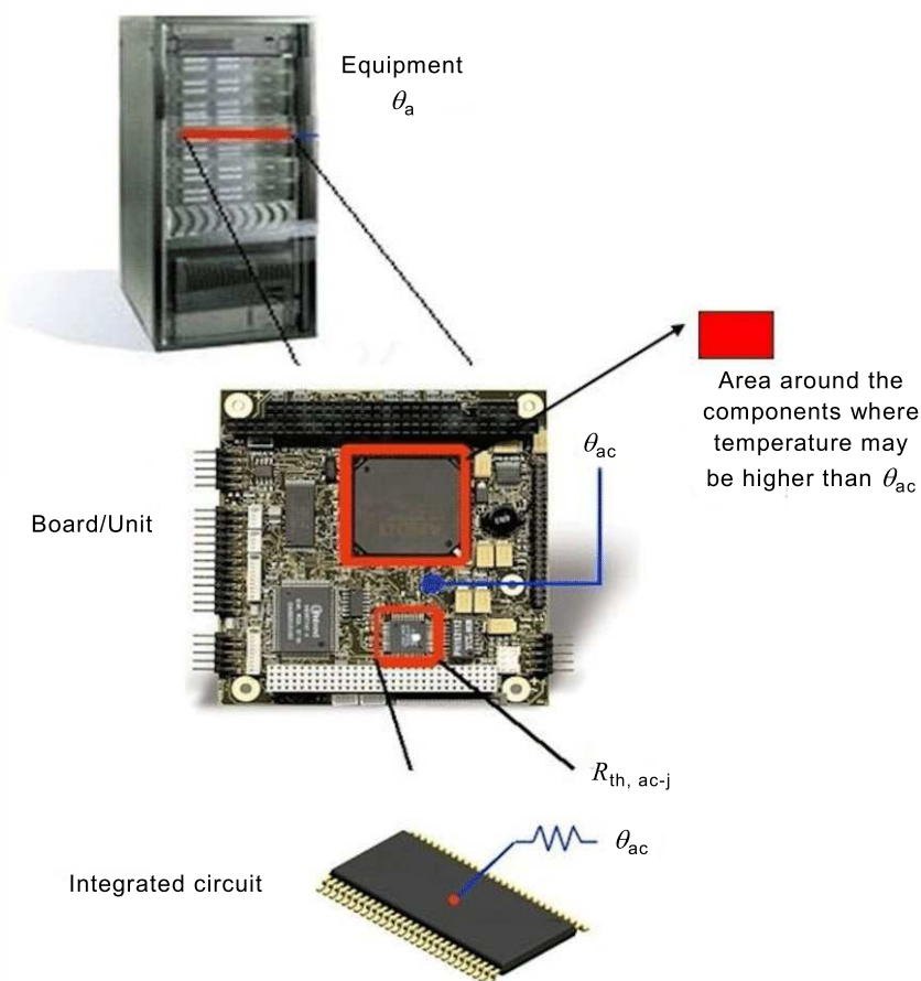
Figure B.1 – Temperatures inside equipment
